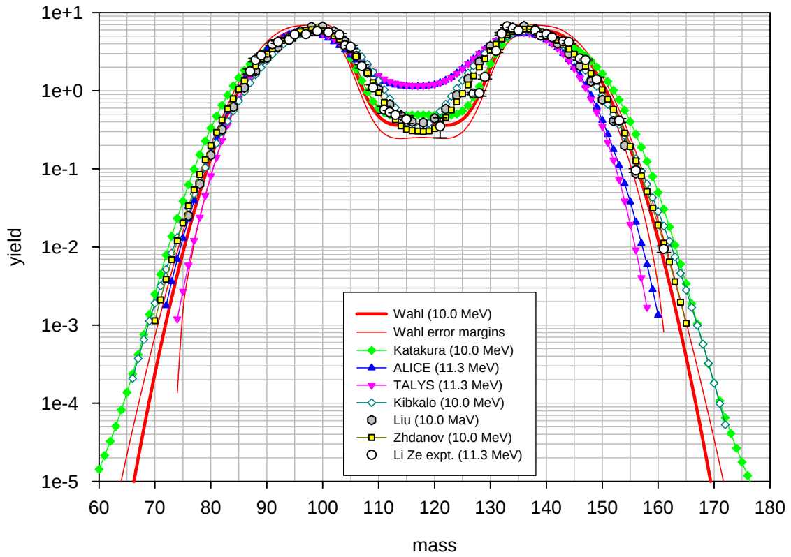
Benchmark A: ^{238}\text{U} at 10.0-11.3 MeV, post neutron emission yields
